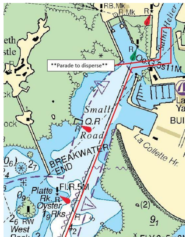
Fig.1. Chartlet highlighting Small Roads/Harbour parade route. Not to be used for Navigation.
