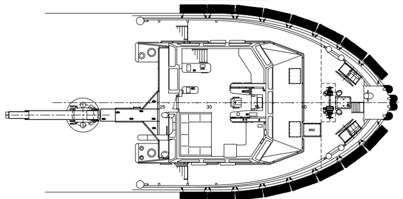
Forecastledeck
